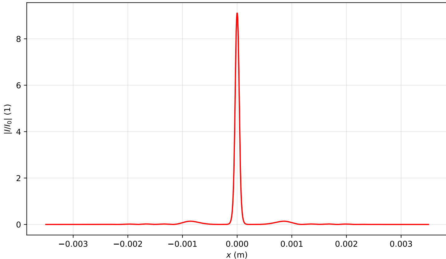
Intensity profile I(x, y = 0, z = 0.637)/I_0 , P_{in}=7.0P_{cr} , artificial time
